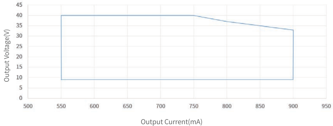
Operating Window
